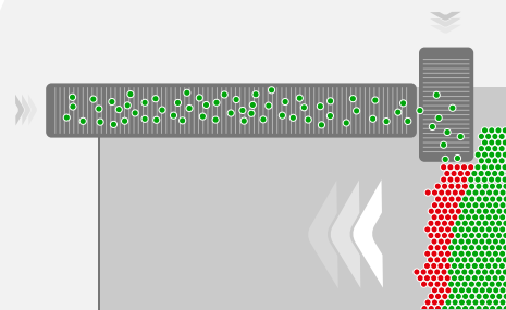
Transversal conveyor belt steadily moves towards the cabin of the machine when the harvested sprouts reach the top of the bunker.
